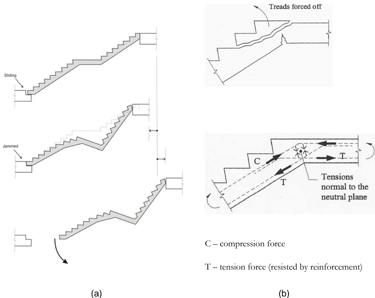
Figure 1: Interstorey drift along the stair: (a) compression forces a shortening of the stair and (b) the knee of the stair/landing “opens” and the landing fails.
