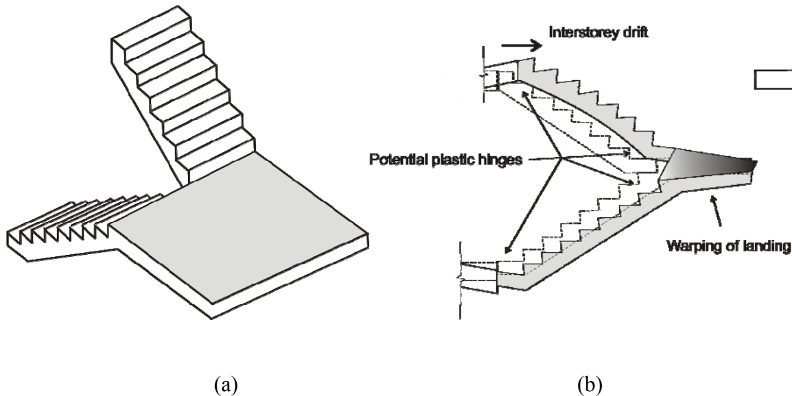
Figure 3: Scissor Stairs
